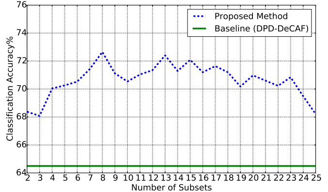
Fig. 3: Performance of the proposed method on the Caltech-UCSD CUB200-2011 bird dataset, while exploiting part annotations. The number of subsets ( K ) is varied from 2 to 25. The subsets are selected automatically. Performance of the baseline system DPD-DeCAF [6] is also shown.
